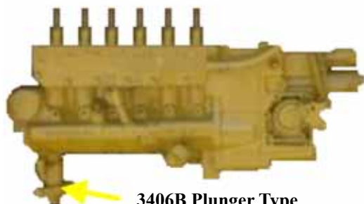
3406B Plunger Type Transfer Pump
