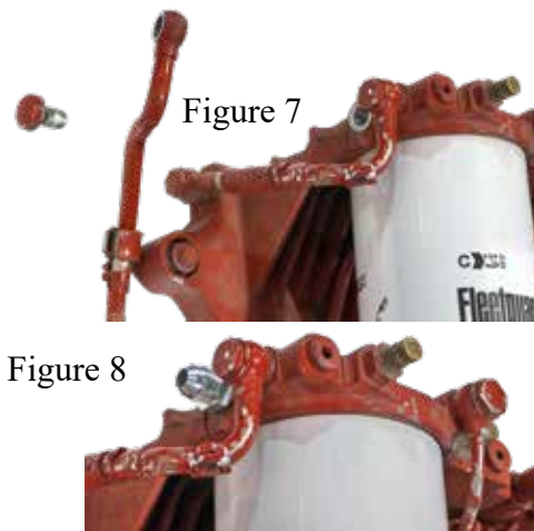
Factory Banjo Bolt
