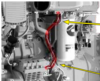
Provided Banjo Fitting (PN 001-4A-1-0031)
